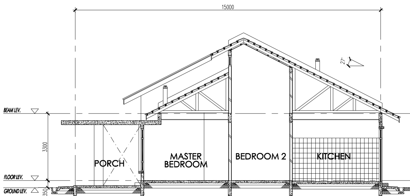
SECTION B-B
