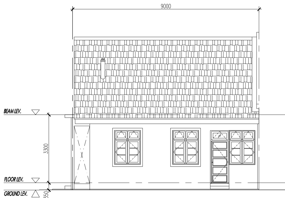
REAR ELEVATION
