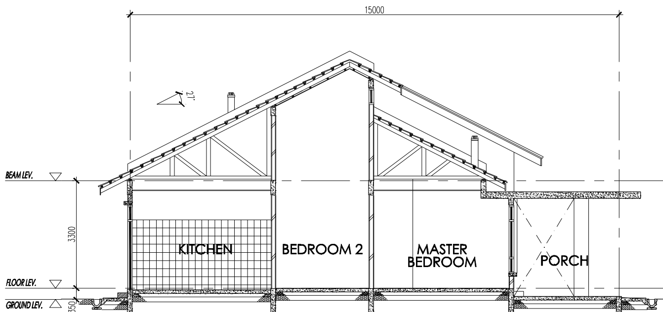
SECTION B-B
