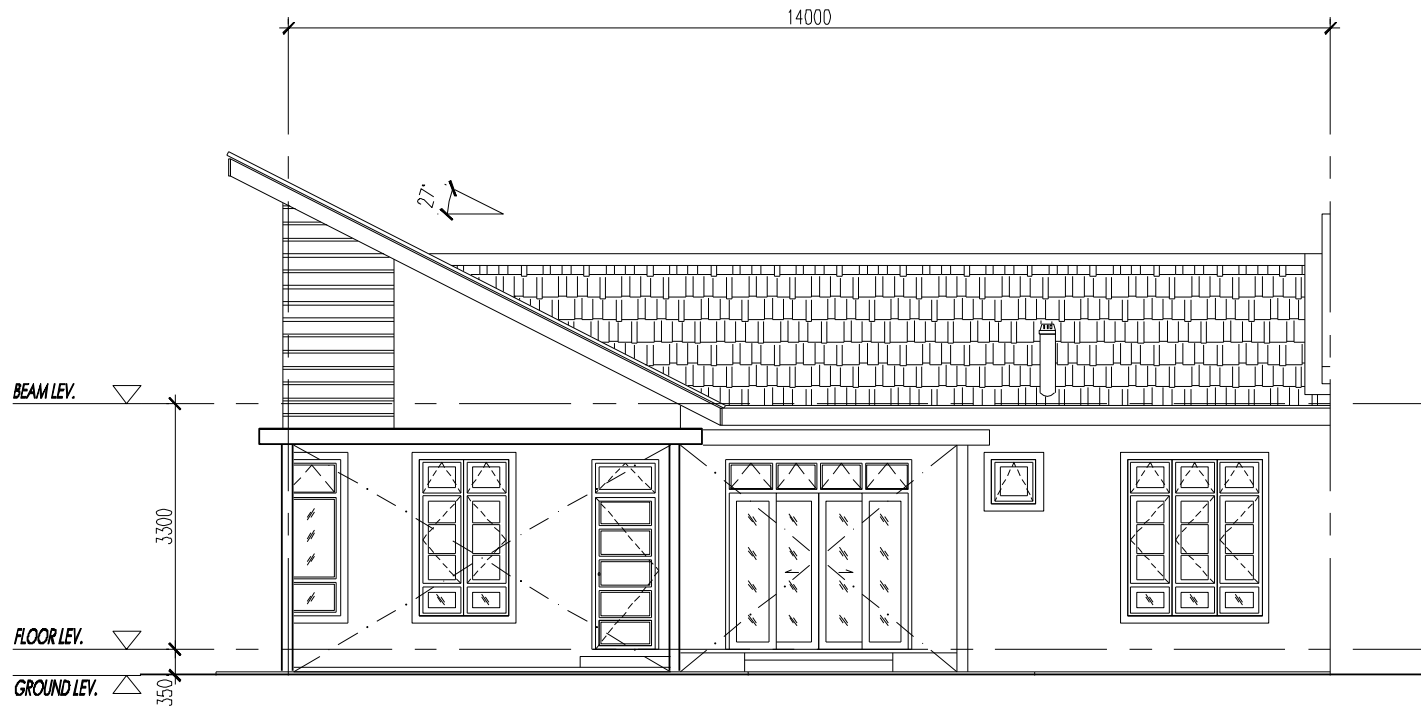
FRONT ELEVATION
