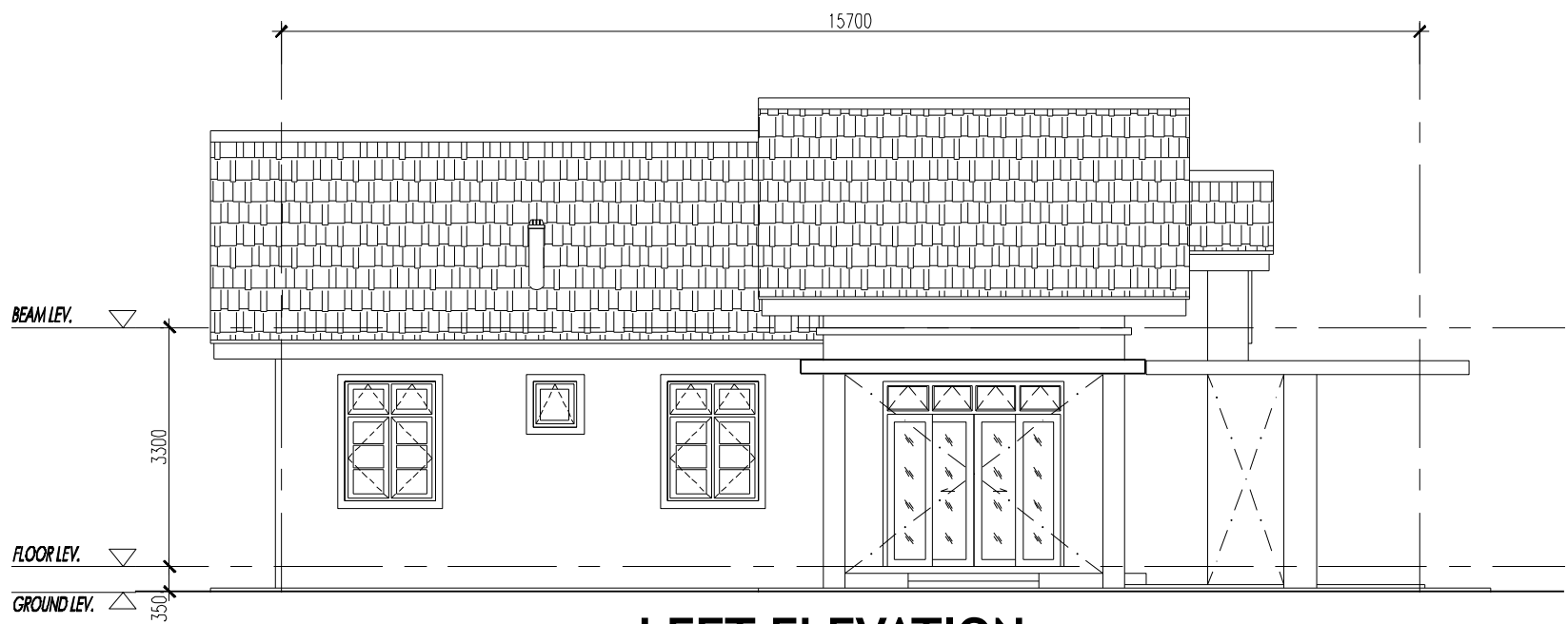
LEFT ELEVATION
