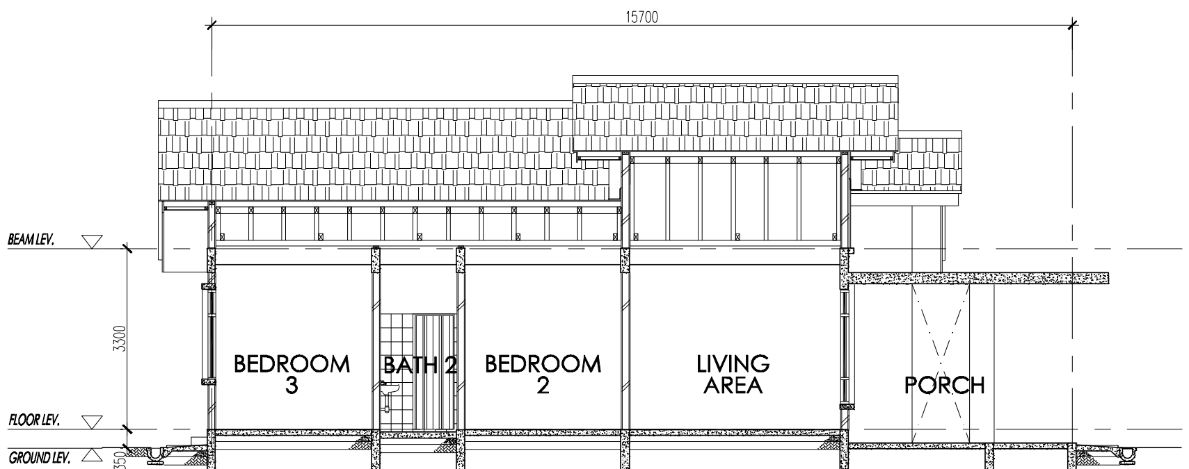
SECTION B-B
