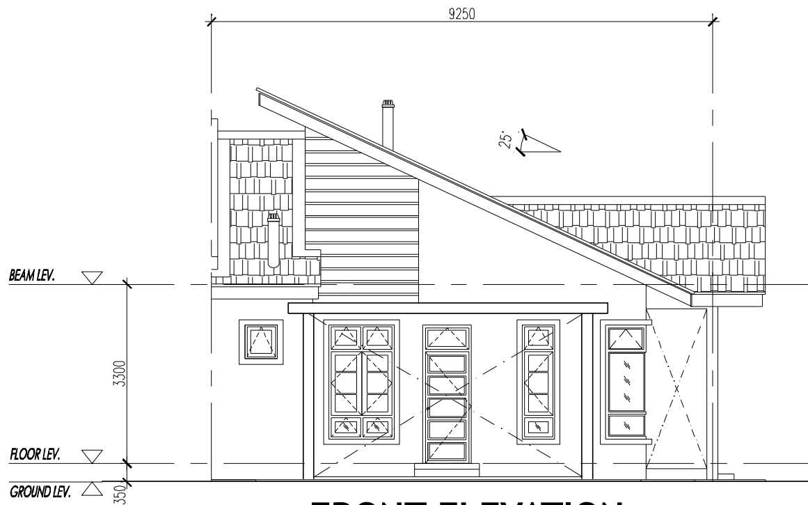
FRONT ELEVATION
