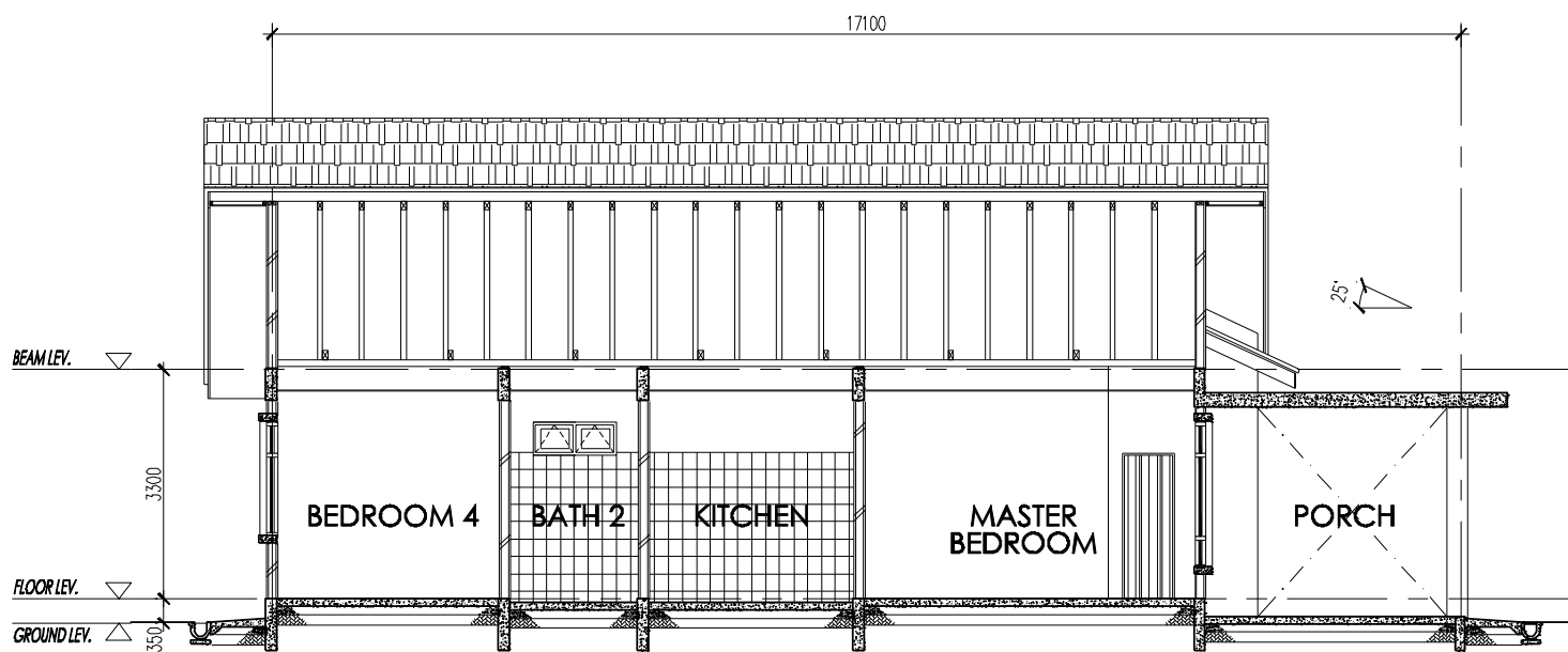
SECTION B-B
