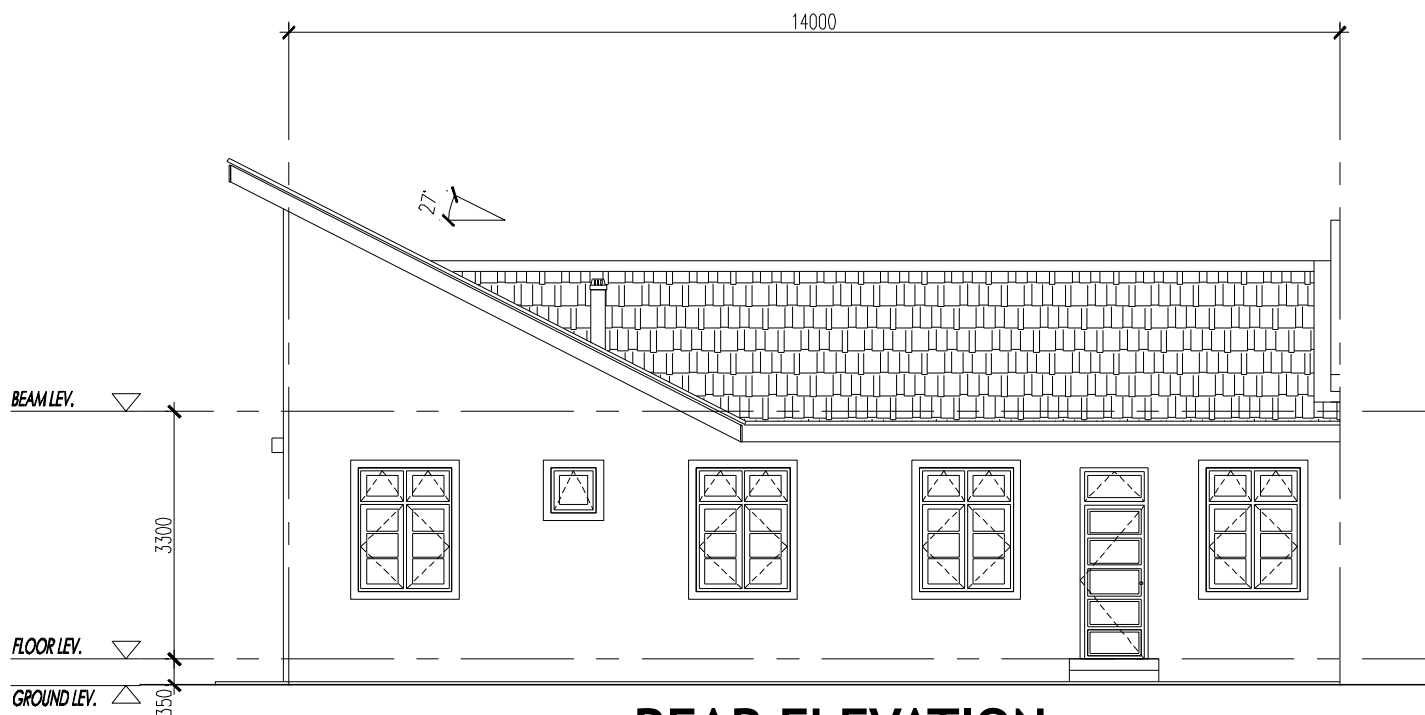
REAR ELEVATION
