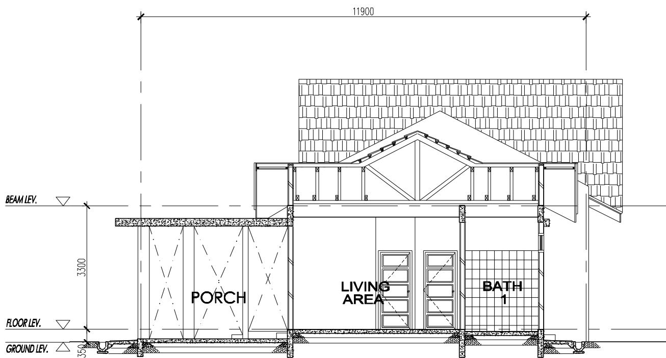
SECTION B-B
