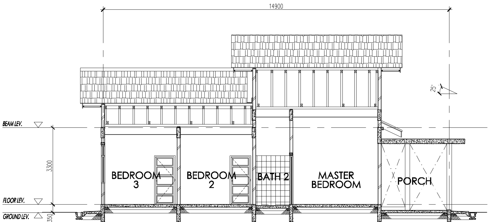
SECTION B-B
