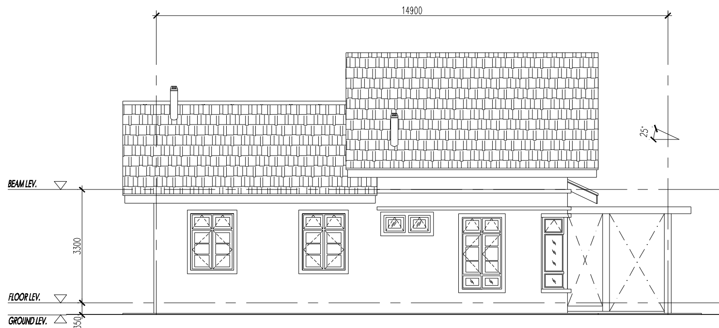
LEFT ELEVATION
